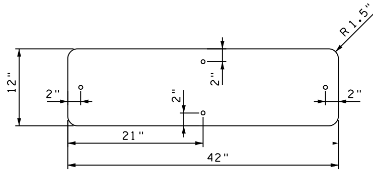
42" x 12" SIGN BLANK WITH 3/8" HOLES
